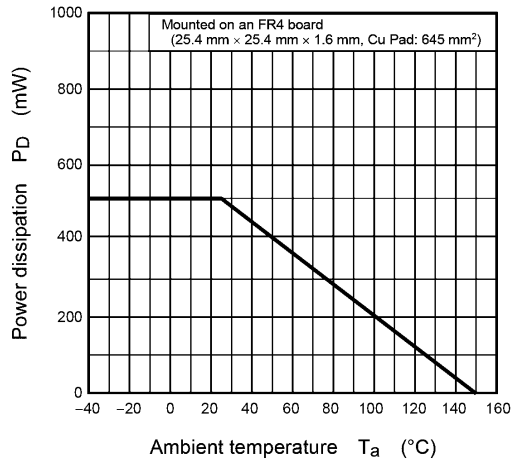
Fig. 8.13 P_D - T_a
