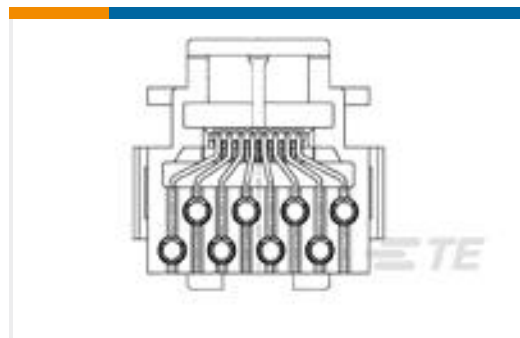
TE Part #216005-4 WITH STUFFER CAP
