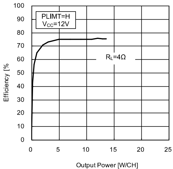
Figure 9. Efficiency vs Output Power (4Ω)
