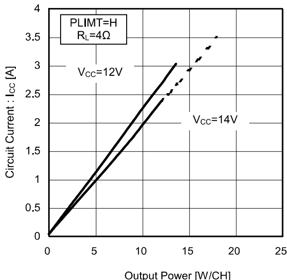
Figure 18. Circuit Current vs Output Power (4Ω)
