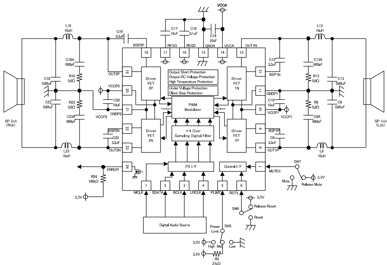
Figure 69. Application Circuit
