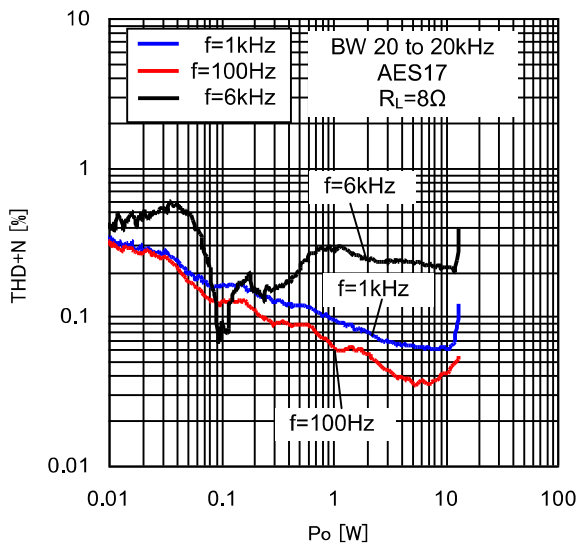
Figure 23. THD+N vs P_o (8Ω)
