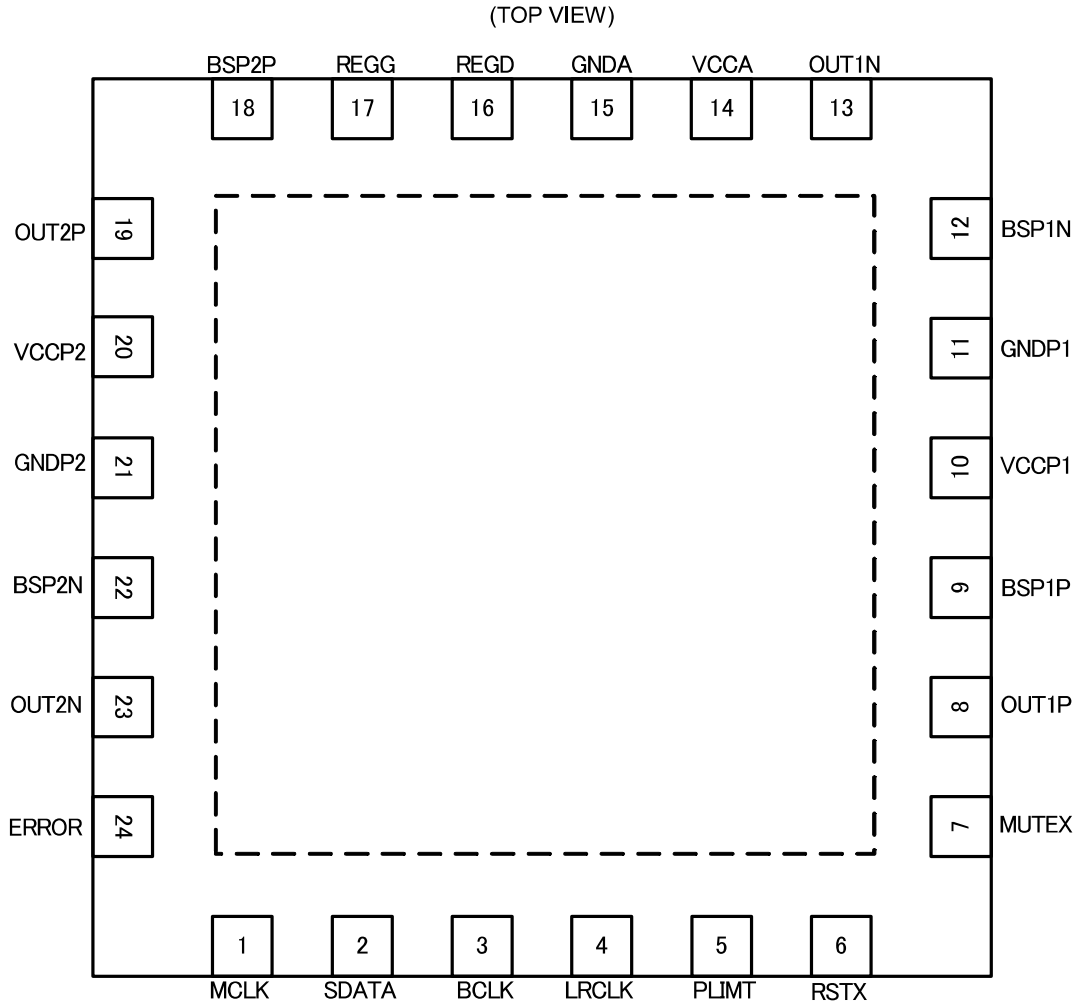
Figure 2. Pin Configuration
