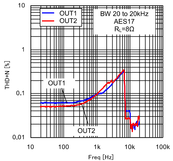
Figure 24. THD+N vs Freq (8Ω)
