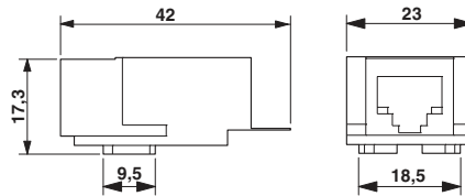
RJ45 socket insert, Freetnet system
