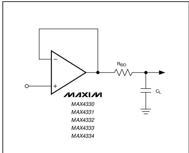
Figure 6. Capacitive-Load-Driving Circuit
