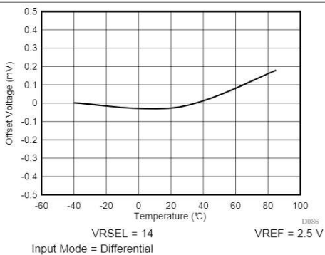
Figure 5-66. Offset Voltage vs Temperature
