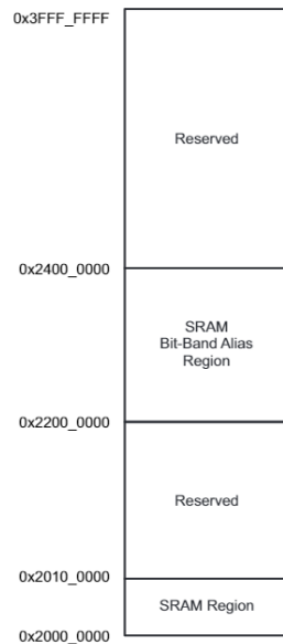
Figure 6-3. SRAM Zone Memory Map
