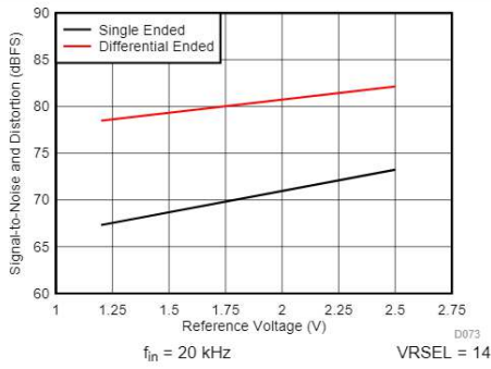
Figure 5-53. SINAD vs Reference Voltage
