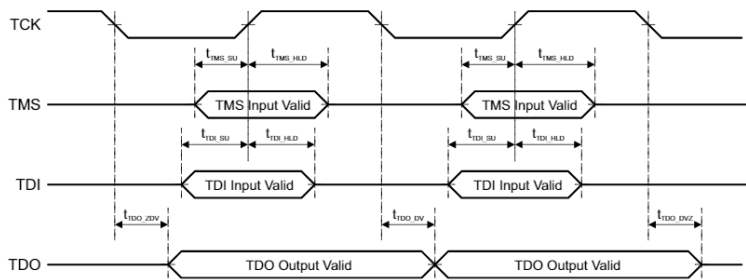
Figure 5-75. JTAG Test Access Port (TAP) Timing
