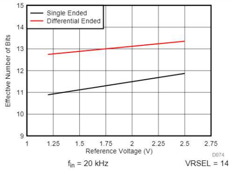
Figure 5-54. ENOB vs Reference Voltage
