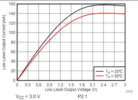
Figure 5-24. Low-Level Output Voltage vs Low-Level Output Current
