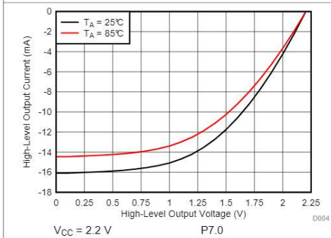
Figure 5-21. High-Level Output Voltage vs High-Level Output Current
