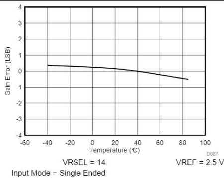
Figure 5-67. Gain Error vs Temperature
