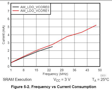
Figure 5-2. Frequency vs Current Consumption
