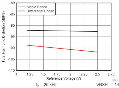
Figure 5-55. THD vs Reference Voltage
