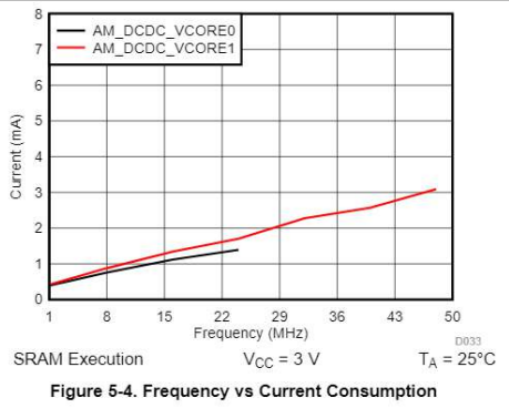
Figure 5-4. Frequency vs Current Consumption
