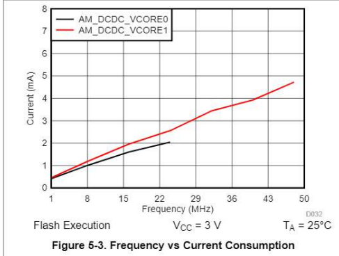
Figure 5-3. Frequency vs Current Consumption
