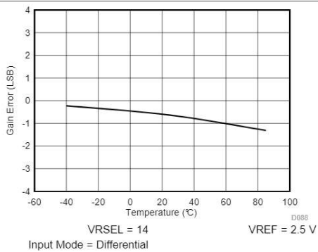
Figure 5-68. Gain Error vs Temperature
