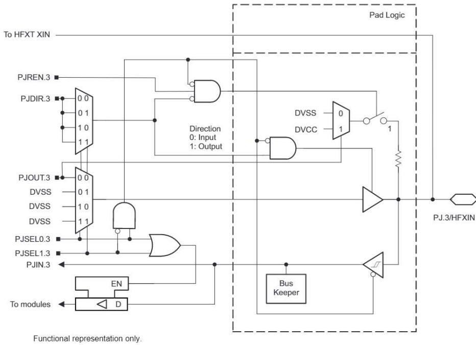
Figure 6-18. Port PJ (PJ.2) Diagram
