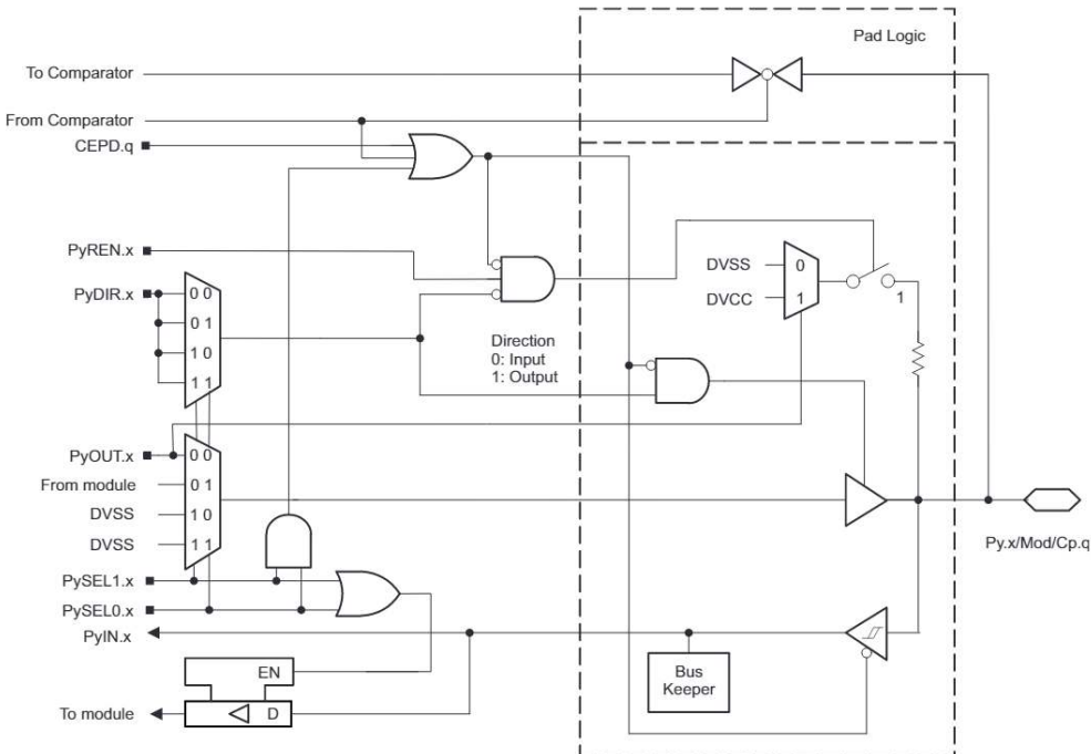
Figure 6-15. Py.x/Mod/Cp.q Pin Diagram
