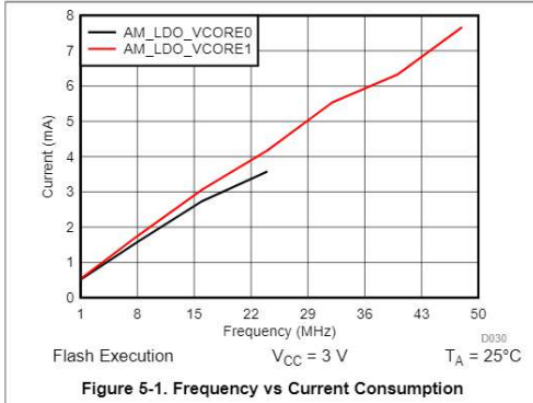
Figure 5-1. Frequency vs Current Consumption
