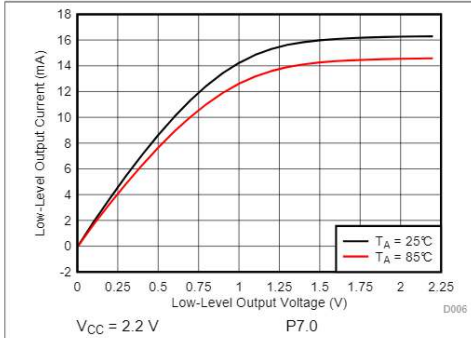
Figure 5-19. Low-Level Output Voltage vs Low-Level Output Current
