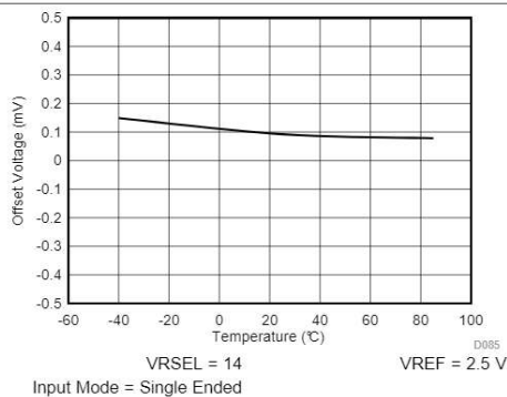
Figure 5-65. Offset Voltage vs Temperature
