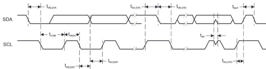
Figure 5-73. I 2 C Mode Timing
