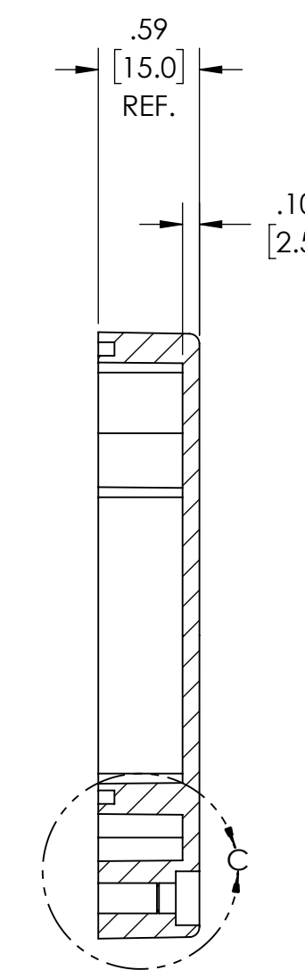
SECTION B-B
