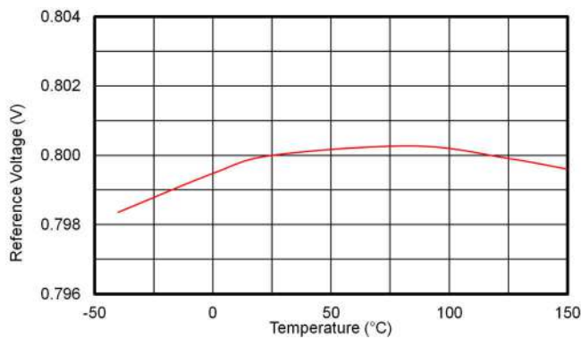
Figure 7-11. Reference Voltage
