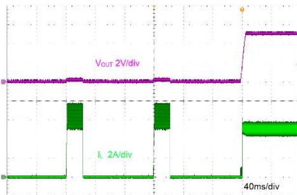
Figure 9-9. Short Recovery
