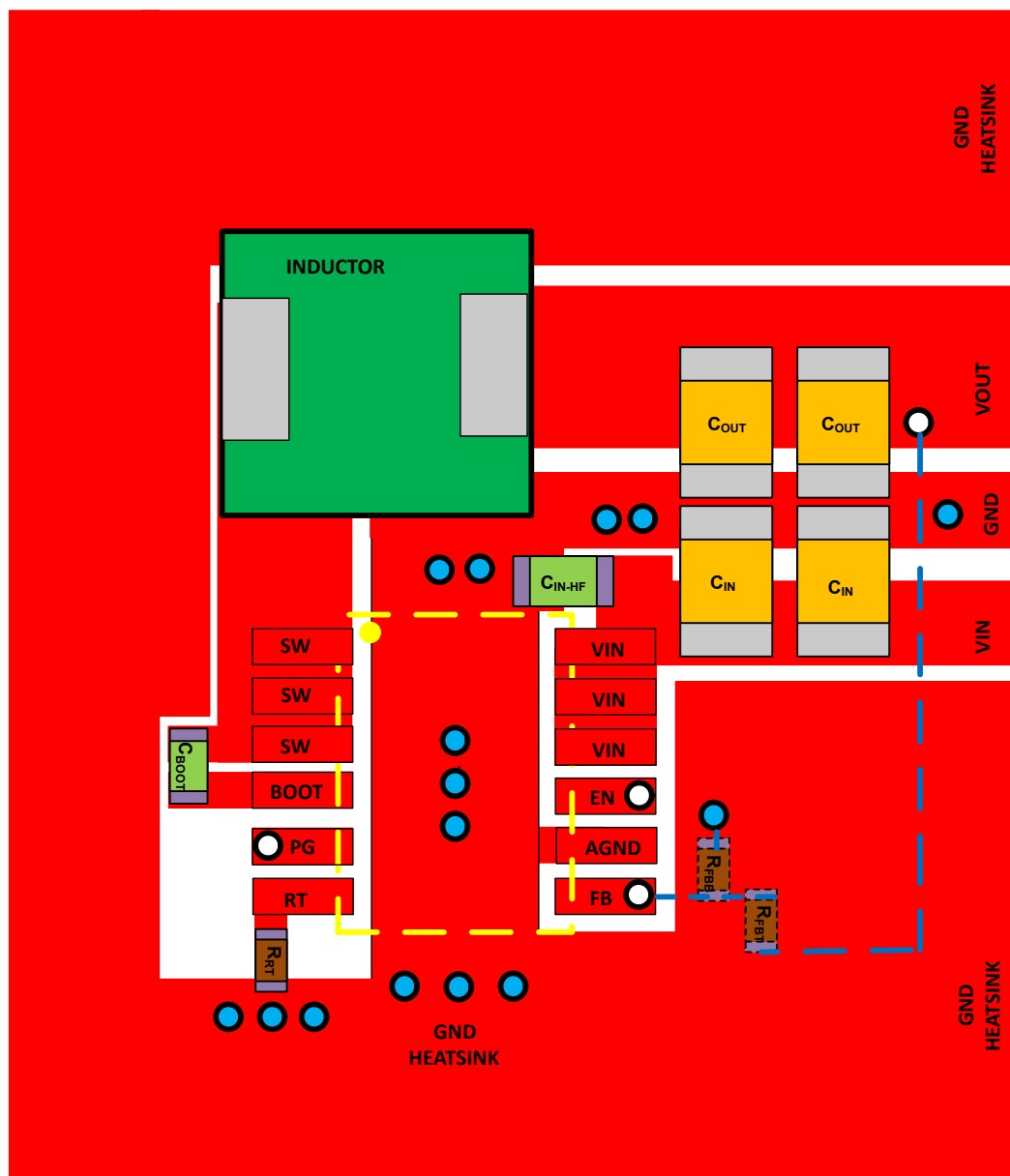
Figure 9-10. Layout
