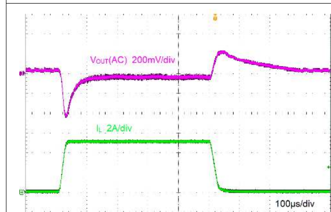
Figure 9-6. Load Transient
