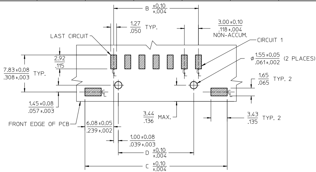
PCB LAYOUT: COMPONENT SIDE 4-12 CKT CONFIGURATION
