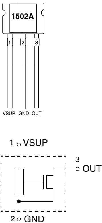
Fig. 4–5: Pin configuration
