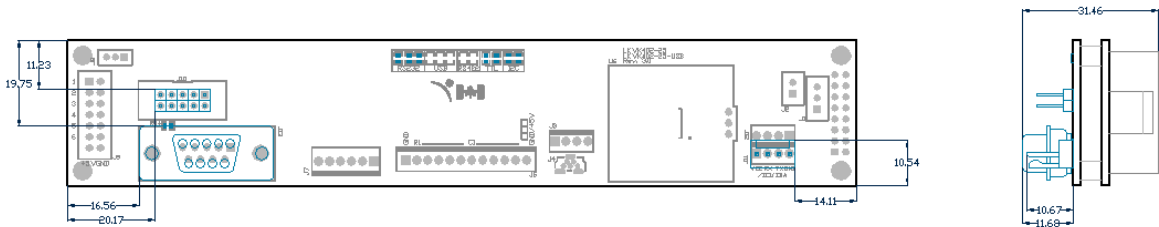
Figure 22: Standard Model Dimensional Drawing
