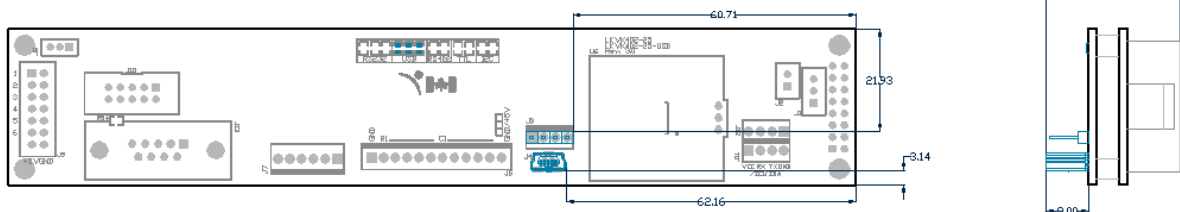
Figure 23: USB Model Dimensional Drawing
