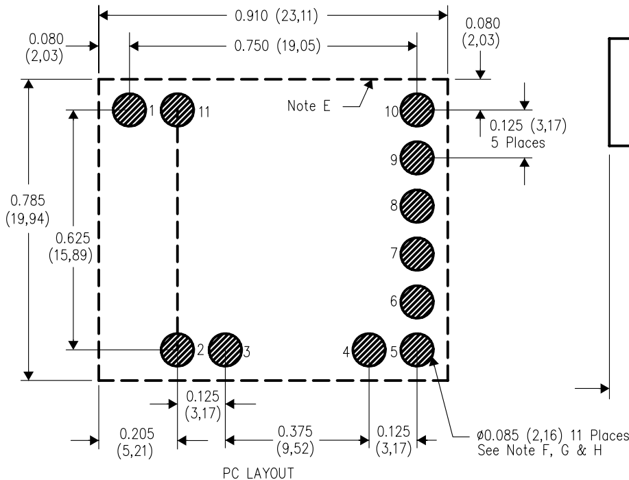
PC LAYOUT
