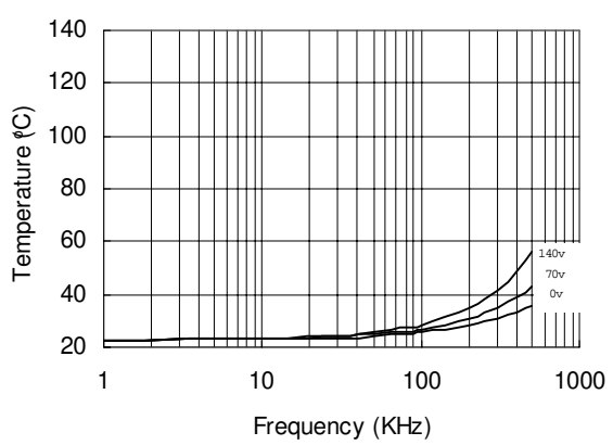
Figure 26. IR2183 vs. Frequency (IRFBC20), R_{gate}=33\Omega, V_{CC}=15V
