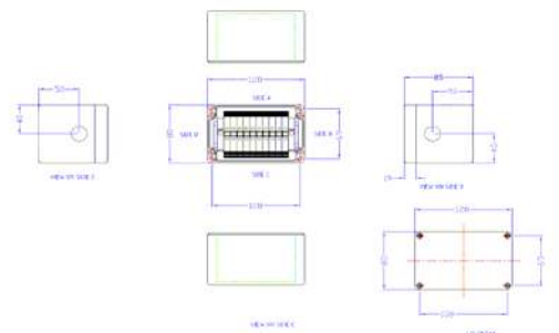
JB-FT10 Drawing
