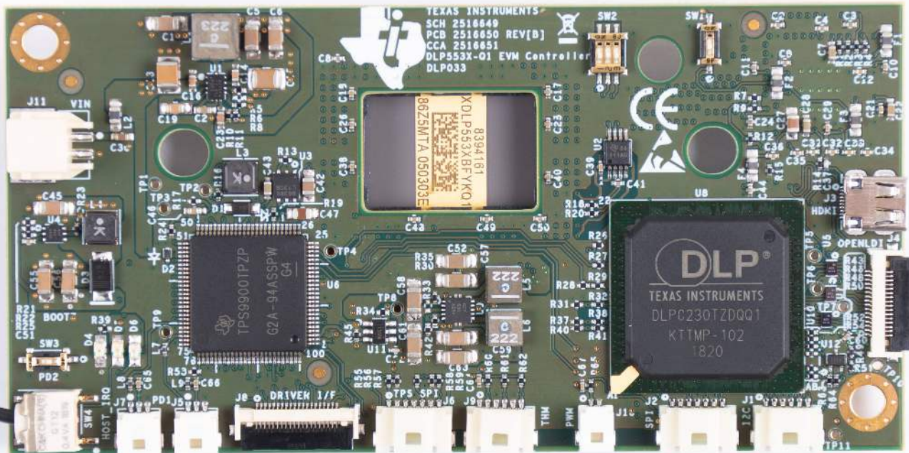
Figure 2. DLP5530PROJQ1EVM Controller PCB
