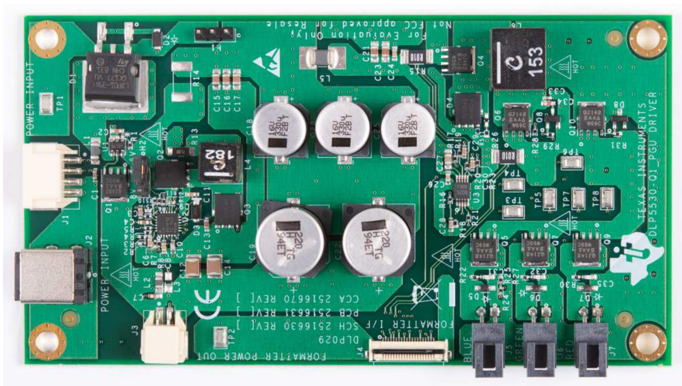
Figure 3. DLP5530PROJQ1EVM Illumination Driver PCB
