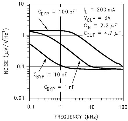
Output Noise Density (LP2988)
