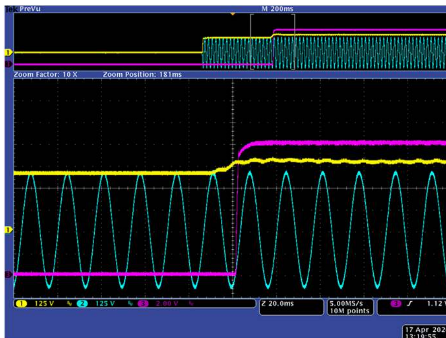
Figure 15. 230Vrms Startup into Full Load Zoomed In (CH1=PFC Output; CH2=AC Input; CH3=LLC Output)
