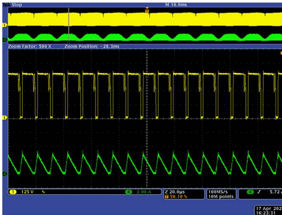
Figure 22. 230Vrms Input, Full Load (CH1=PFC Switch Node; CH4=PFC Inductor Current)
