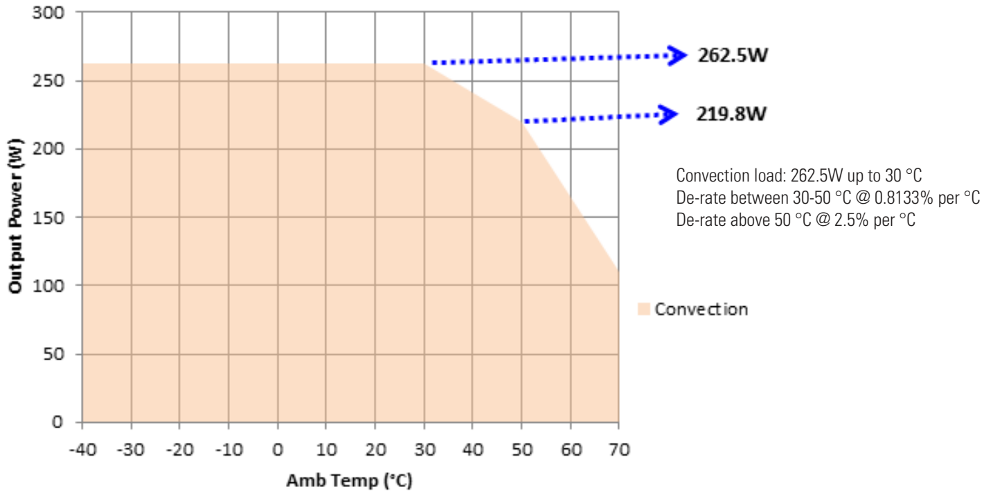
Derating Curve 15 V slotted cover
