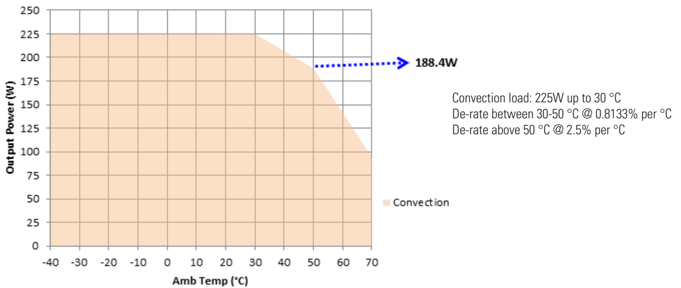
Derating Curve 15 V plain cover
