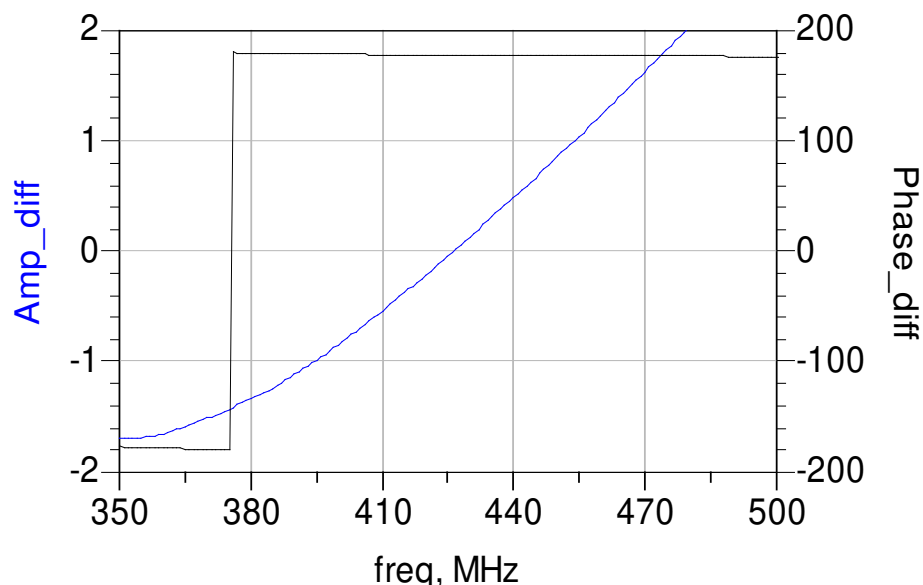
Amplitude and Phase Balance
