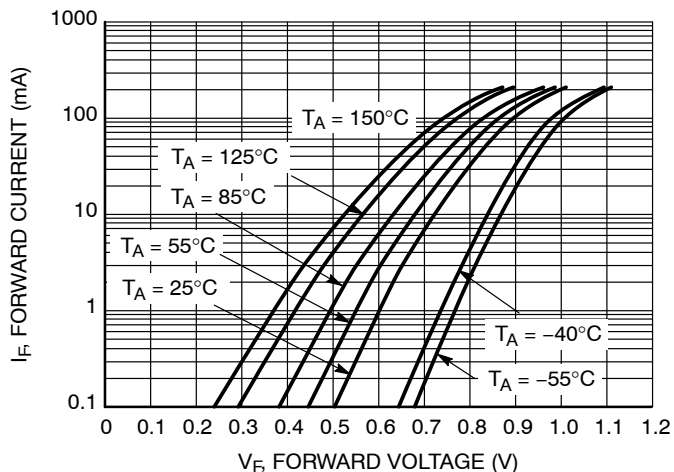
Figure 12. Forward Voltage
