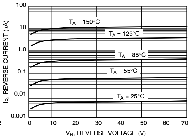
Figure 13. Leakage Current
