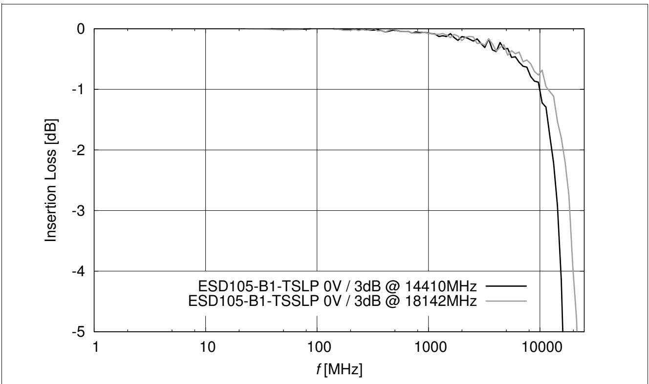
Figure 14 Insertion loss vs. frequency of ESD105-B1-02xx in a 50 Ω system
