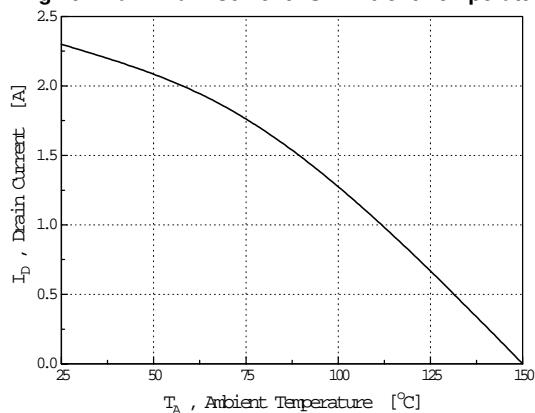
Fig 10. Max. Drain Current vs. Ambient Temperature
