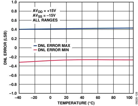
Figure 13. Differential Nonlinearity Error vs. Temperature
