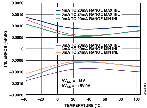
Figure 37. Integral Nonlinearity vs. Temperature, External RSET
