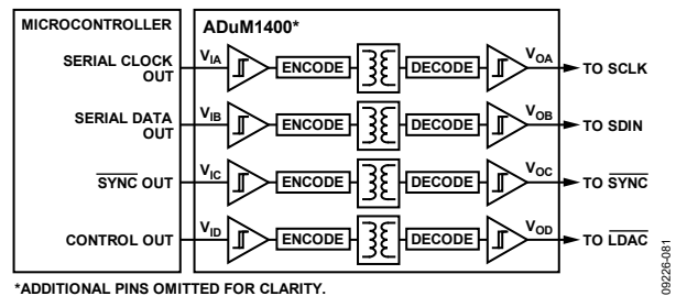
Figure 89. Isolated Interface
