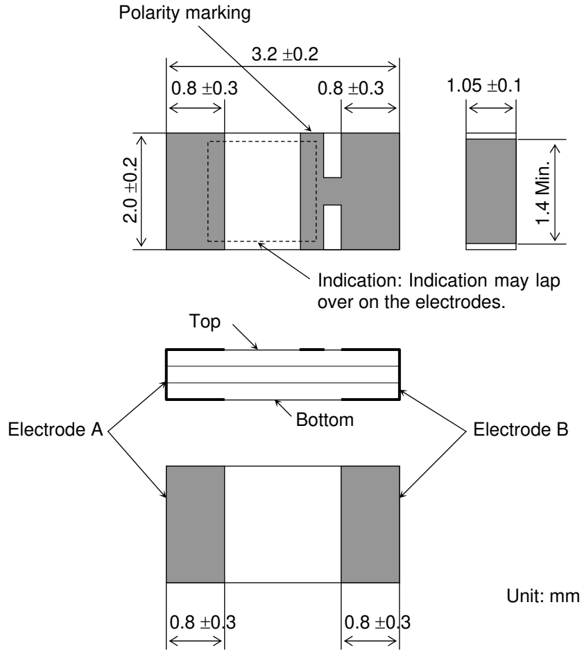
Figure 2. Dimensions
