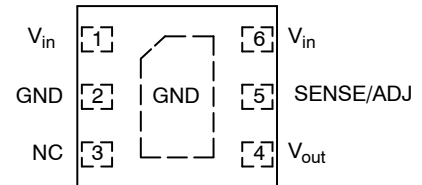
NCV8605, DFN6 3x3.3mm (Top View)
