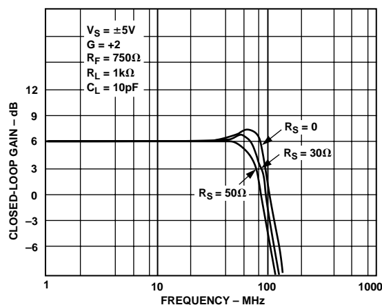
Figure 42. Response to a Small Load Capacitor at \pm 5\text{ V}
