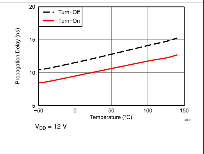
Figure 14. Input to Output Propagation Delay vs Temperature
