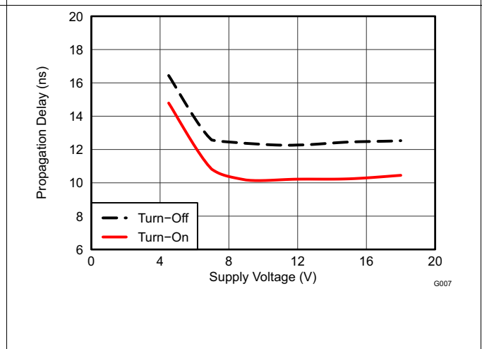
Figure 16. Propagation Delays vs Supply Voltage
