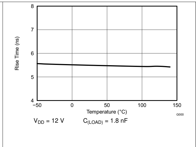
Figure 12. Rise Time vs Temperature
