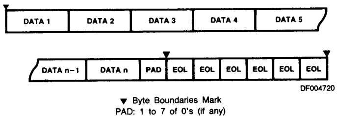
Figure 55. No Byte Boundary Conditioned without EOL and Time Fill
