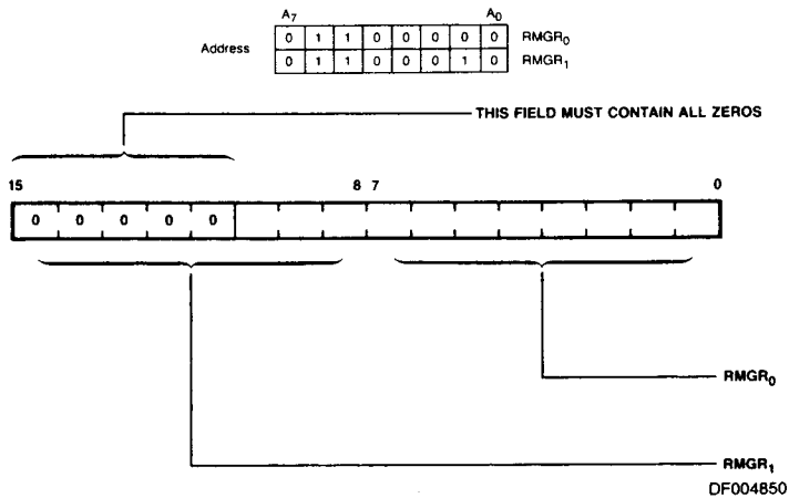
Figure 31. Right Margin Register (RMGR)
