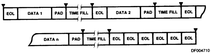
Figure 54. Byte Boundary Conditioned with Auto EOL and Time Fill
