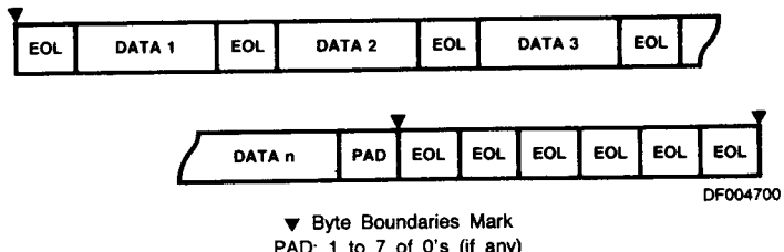
Figure 53. No Byte Boundary Conditioned with Auto EOL and No Time Fill
