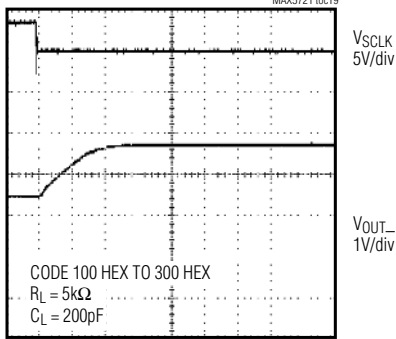
HALF-SCALE SETTLING TIME ( V_{DD} = +3\text{V} )
