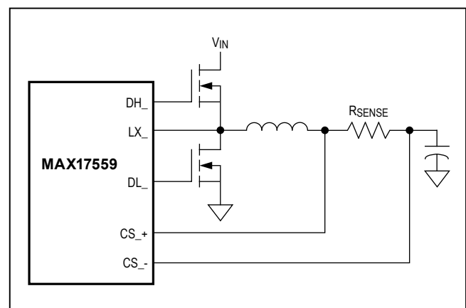
Figure 5. Current Sensing Using an External Sense Resistor
