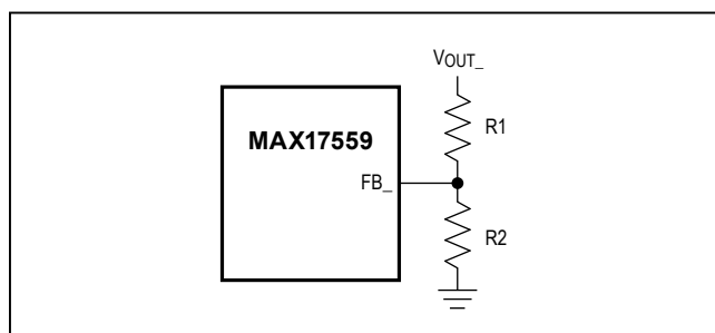
Figure 4. Output-Voltage Programming
