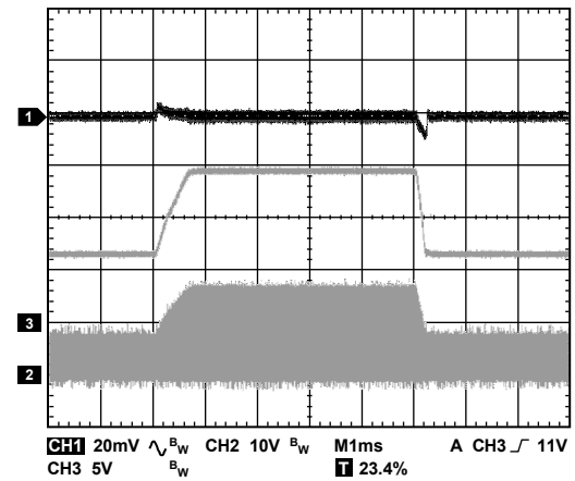
Figure 14. ADP2303 Line Transient, 7 V to 15 V, V_{OUT} = 3.3\text{ V} , I_{OUT} = 3\text{ A} , L = 4.7\text{ }\mu\text{H} , C_{OUT} = 2 \times 47\text{ }\mu\text{F}
