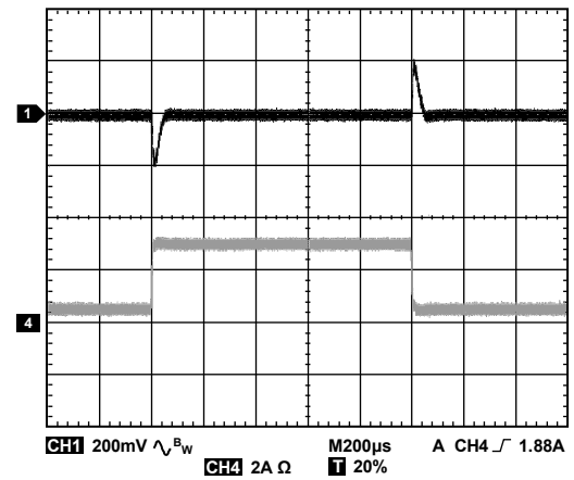
Figure 13. ADP2303 Load Transient, 0.5 A to 3.0 A, V_{OUT} = 3.3\text{ V} , V_{IN} = 12\text{ V} , L = 4.7\text{ }\mu\text{H} , C_{OUT} = 2 \times 47\text{ }\mu\text{F}
