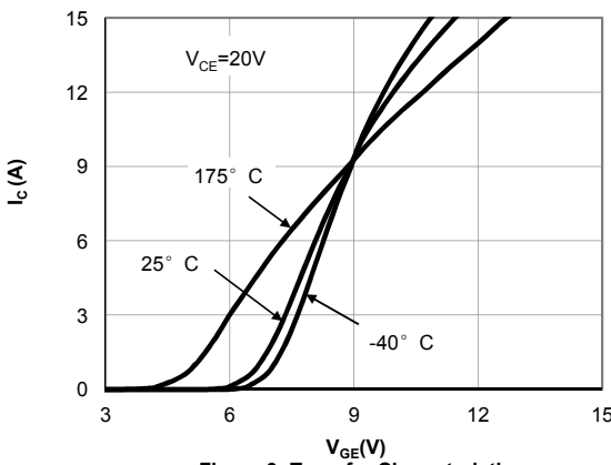
Figure 3: Transfer Characteristic
