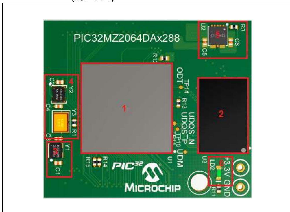
FIGURE 1-4: PIC32MZ2064DAx288 DAUGHTER CARD LAYOUT (TOP VIEW)
