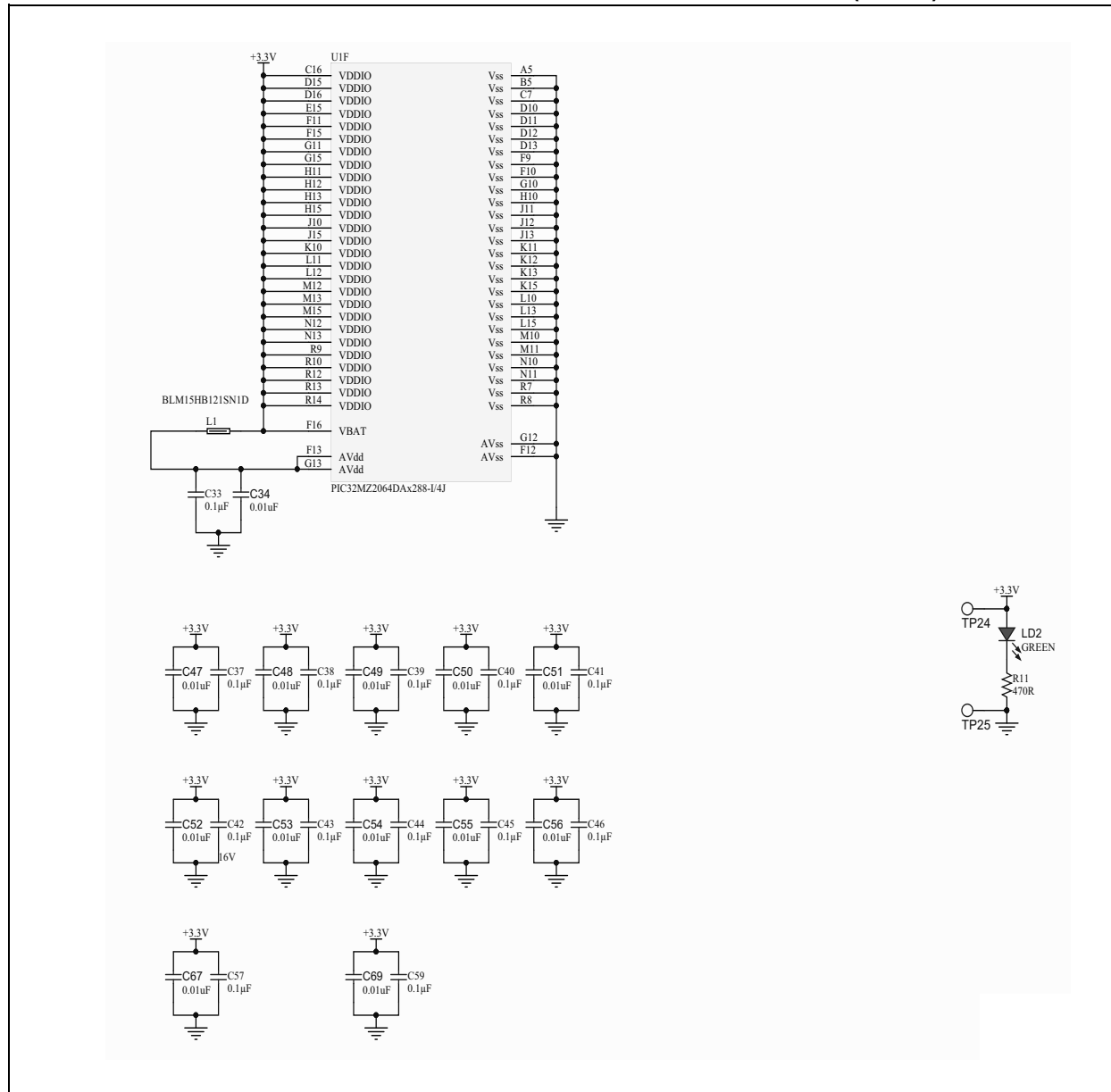
FIGURE A-4: PIC32MZ2064DAX288 DAUGHTER CARD SCHEMATICS (4 OF 4)
