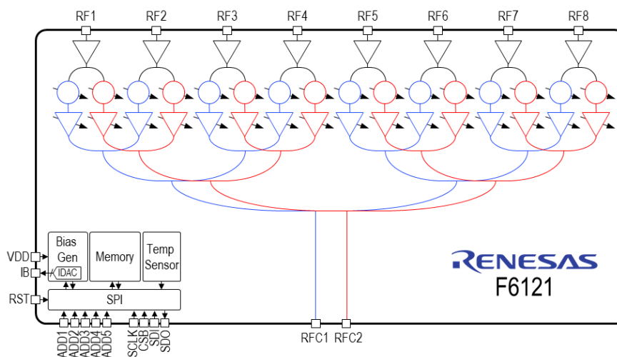
Figure 1. Block Diagram
