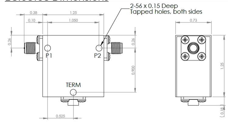
D3I0810S-3 Dimensions
