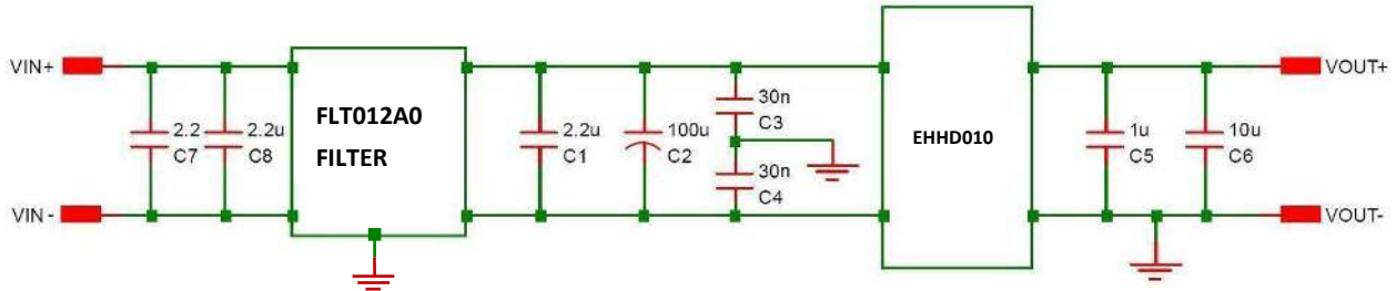
Figure 27. EMC Considerations
