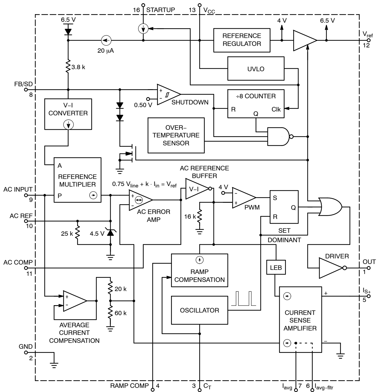
Figure 1. Block Diagram
