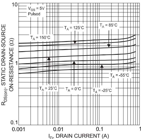
Fig. 5 Static Drain-Source On-Resistance vs. Drain Current
