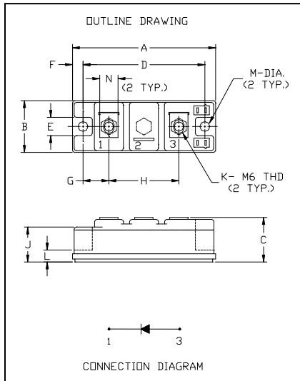
QRS1240T30 Fast Recovery Diode Module
