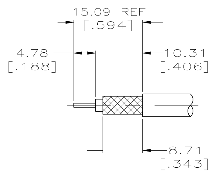
VIEW U RECOMMENDED STRIP LENGTH
