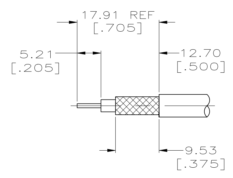
VIEW X RECOMMENDED STRIP LENGTH
