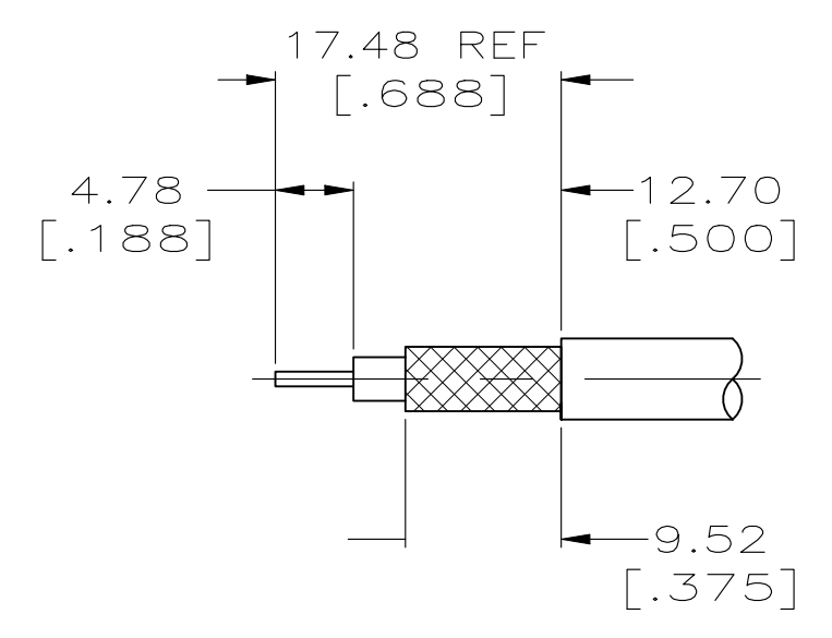
VIEW V RECOMMENDED STRIP LENGTH
