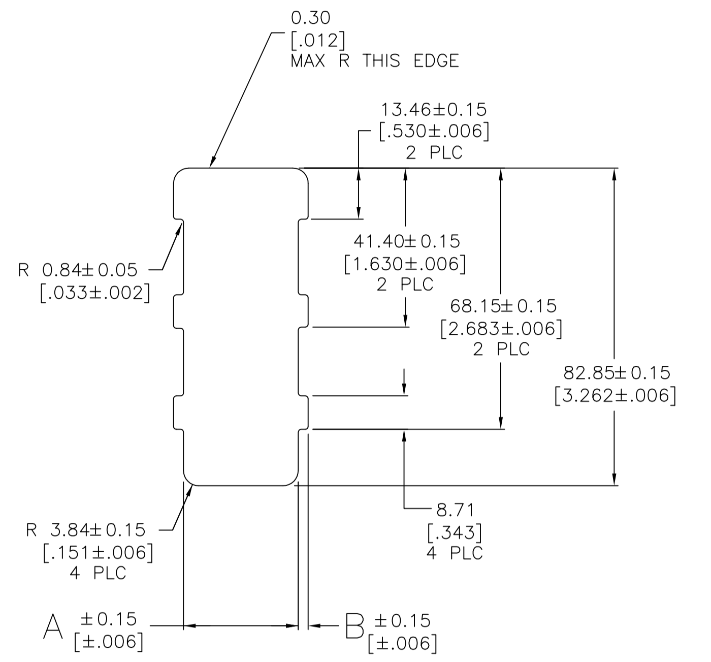
RECOMMENDED PANEL CUTOUT \Delta SCALE 1:1
