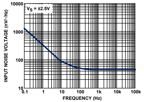
FIGURE 11. VOLTAGE NOISE vs FREQUENCY
