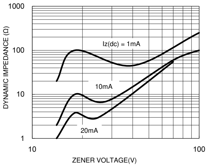
Fig.7 Effect Of Zener Voltage
