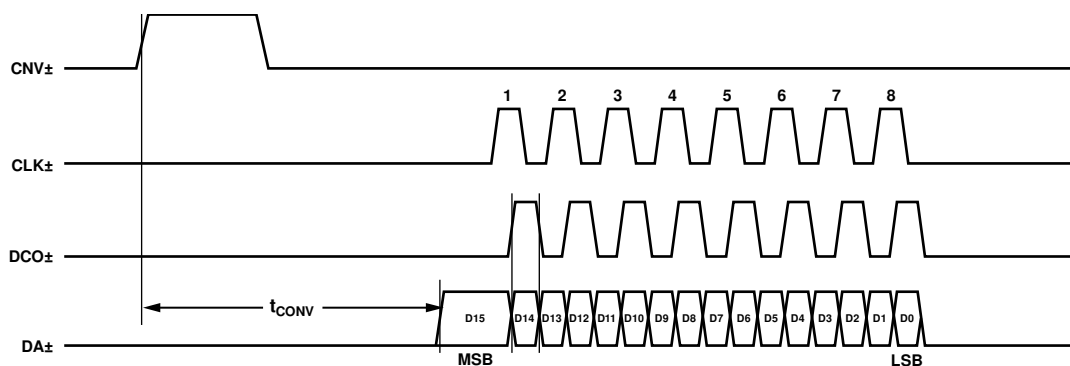
Figure 43. Timing Diagram for a Single Conversion in One-Lane Mode
