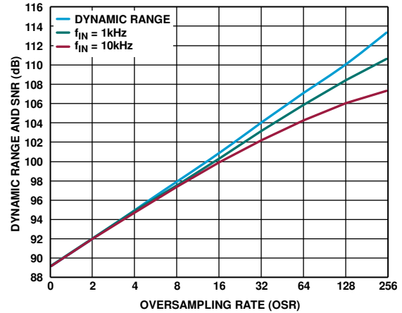
Figure 34. Dynamic Range and SNR vs. Oversampling Rate for Input Frequencies
