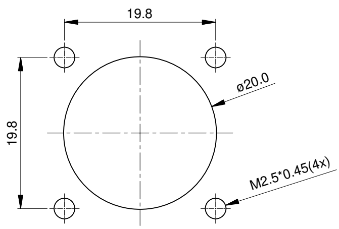
MOUNTING HOLE
