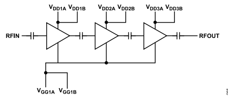
Figure 55. Simplified Internal ADPA7002CHIP Block Diagram
