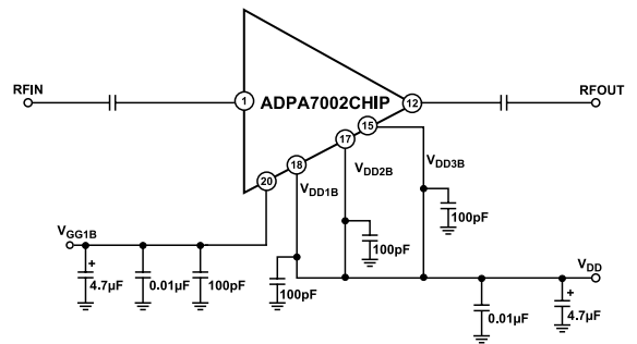
Figure 54. Typical Application Circuit
