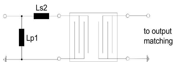
Fig. 3 shunt L – series L matching
