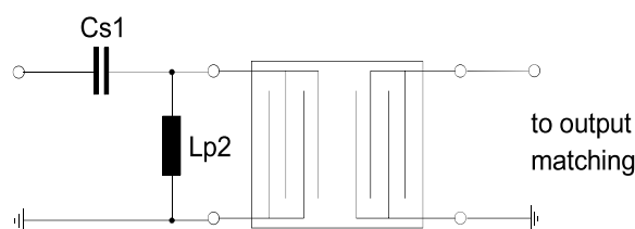
Fig. 4 series C – shunt L matching
