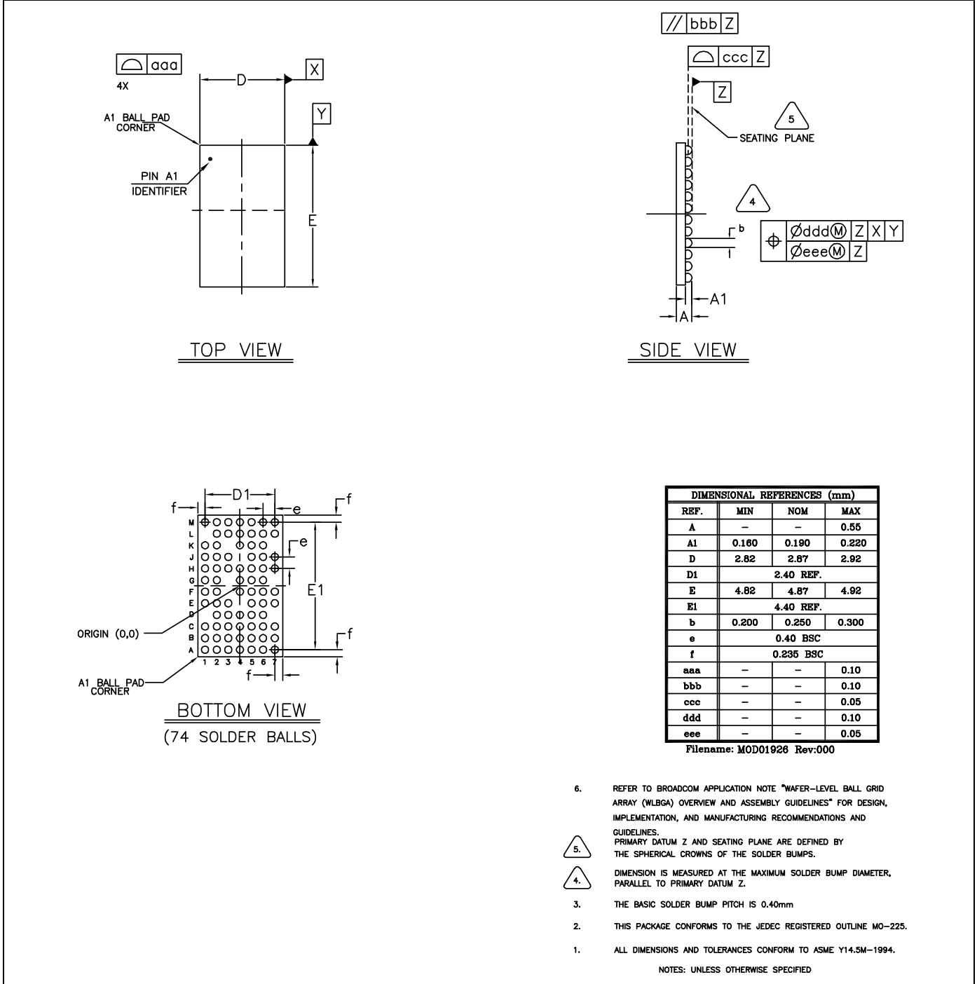
Figure 21. 74-Ball WLBGA Mechanical Information
