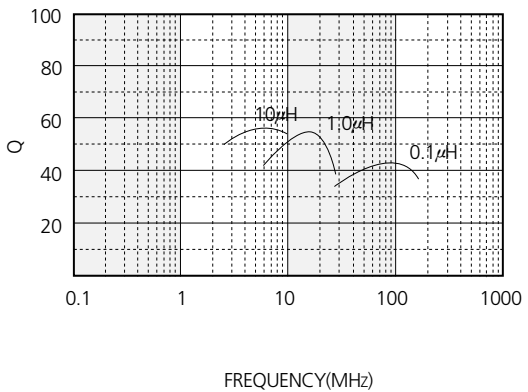
■ Q CHARACTERISTICS
