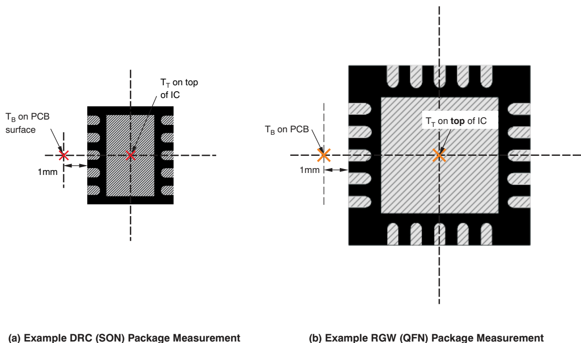
Figure 8-14. Measuring Points for T_T and T_B
